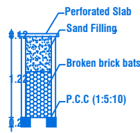
RAIN WATER COLLECTION WELL
