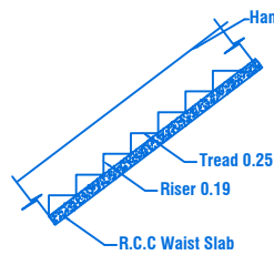
STAIR DETAILS
