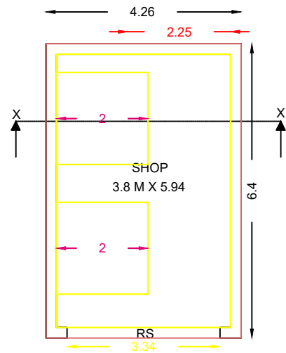
COMMERCIAL GROUND FLOOR PLAN
