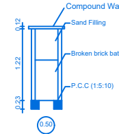
RAIN WATER COLLECTION WELL
