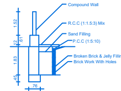
RAIN WATER HARVEST DETAILS
