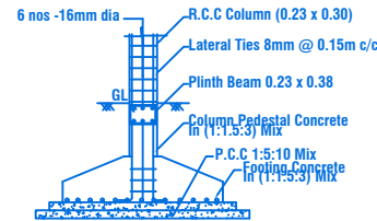
COLUMN FOOTING DETAILS
