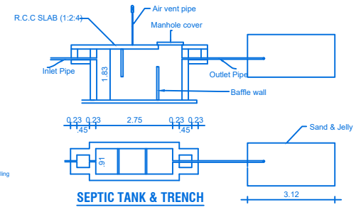
SEPTIC TANK & TRENCH
