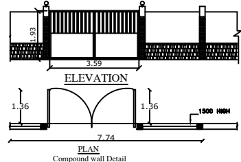
Compound wall Detail
