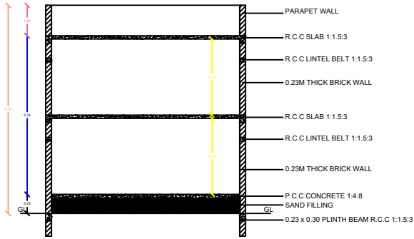
SECTION A- B
