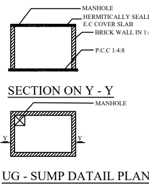
SECTION ON Y - Y UG - SUMP DETAIL PLAN
