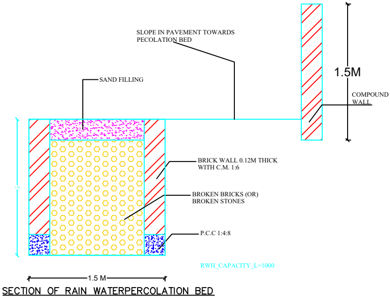
SECTION OF RAIN WATERPERCOLATION BED
