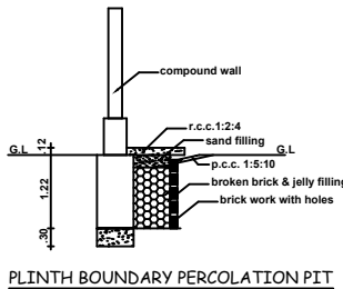
PLINTH BOUNDARY PERCOLATION PIT
