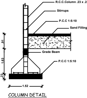
COLUMN DETAIL
