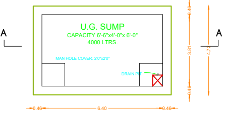
SUMP DETAIL
