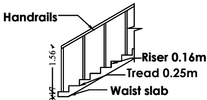
STAIRCASE DETAILS
