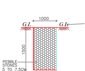
SECTION OF PEBBLE TRENCH
