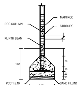
COLUMN DETAILS
