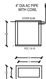
SEPTIC TANK
