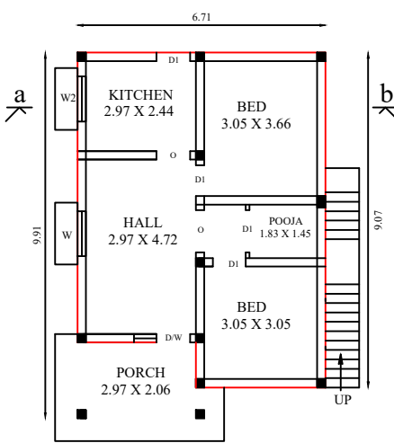
PLAN
