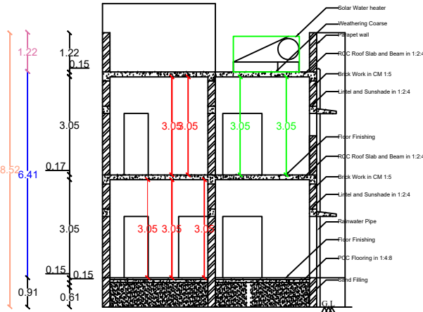
SECTION - "AB"
