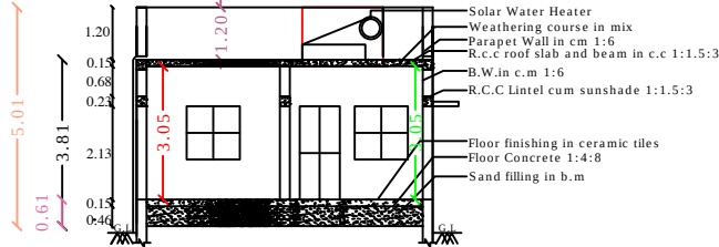
SECTION - "AB "
