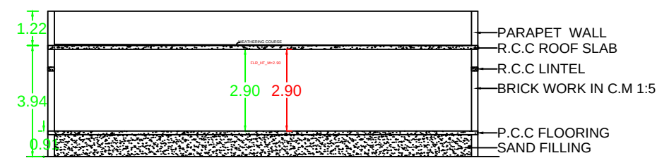
SECTION ON A-A
