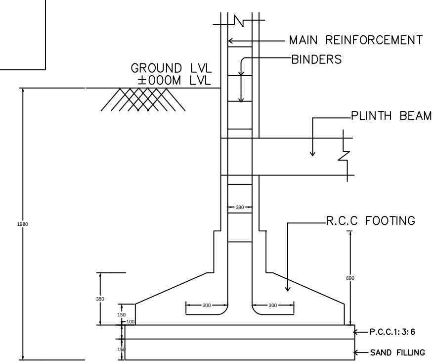
TYPICAL SECTION OF R.C.C COLUMN FOUNDATION SCALE : 1" = 2'-0"
