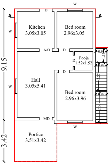
EXI. GROUND FLOOR PLAN
