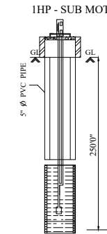
BOREWELL DETAILS
