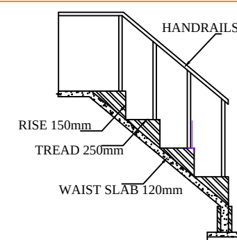
STAIRCASE DETAILS
