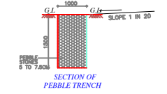
SECTION OF PEBBLE TRENCH
