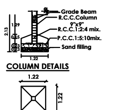
COLUMN DETAILS
