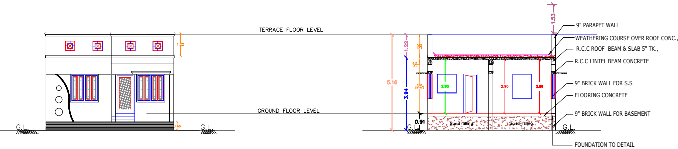
FRONT ELEVATION
