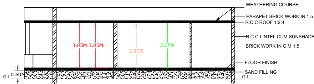
SECTION ON XX
