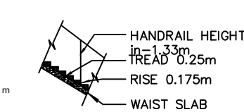
STAIRCASE DETAILS
