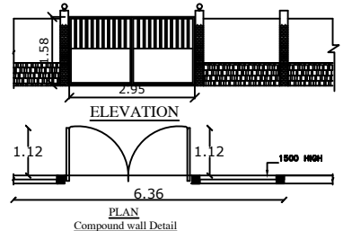
Compound wall Detail
