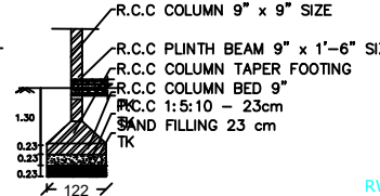
SECTION
