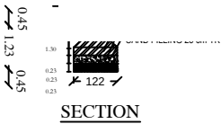
SECTION
