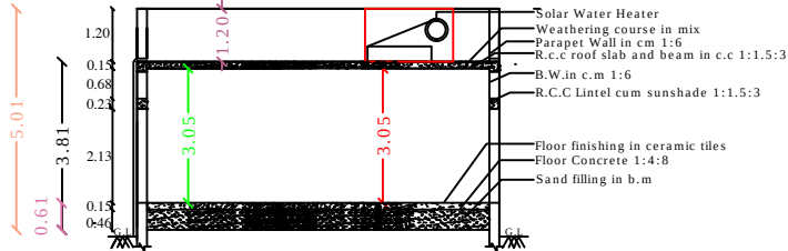
SECTION - "AB "
