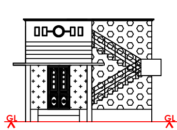
FRONT ELEVATION
