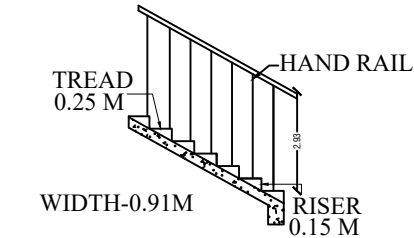
STAIRCASE DETAILS
