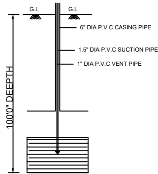
BORE WELL
