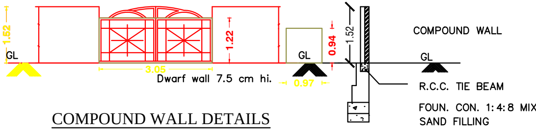
SECTION
