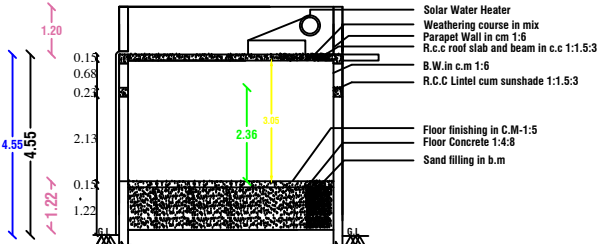
SECTION - "AB "
