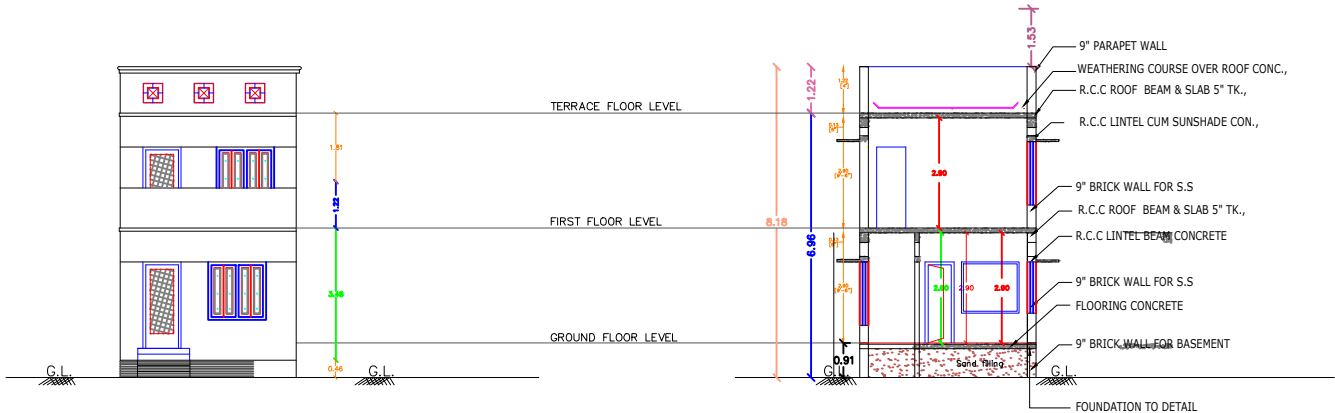
FRONT ELEVATION
