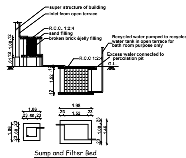
Sump and Filter Bed
