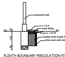
PLINTH BOUNDARY PERCOLATION PIT
