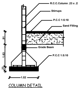
COLUMN DETAIL
