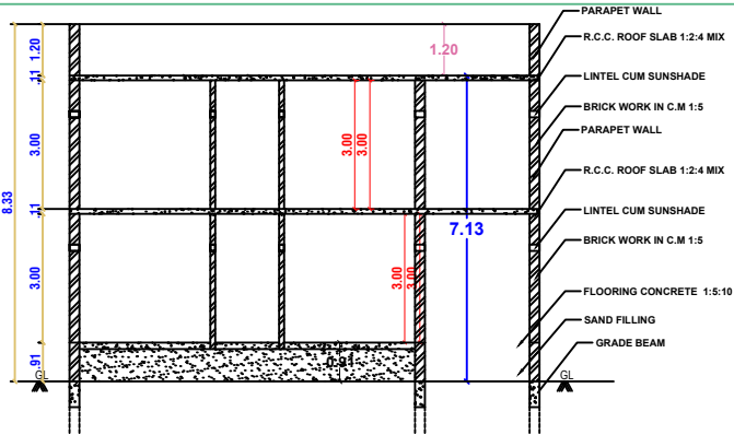
SECTION-AB
