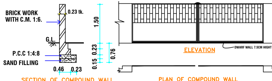
SECTION OF COMPOUND WALL
