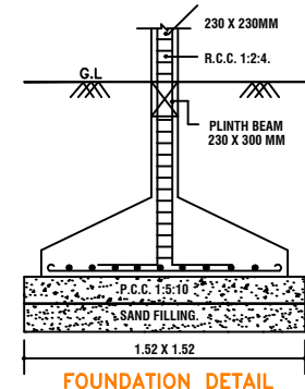
FOUNDATION DETAIL
