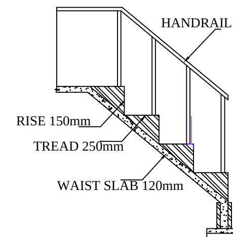
STAIRCASE DETAILS
