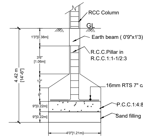
FOUNDATION DETAILS
