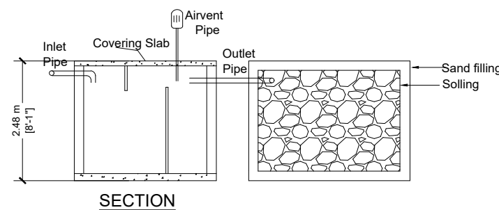
DETAILS OF SEPTIC TANK & DISPERSION TRENCH
