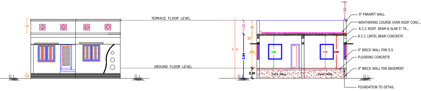
FRONT ELEVATION
