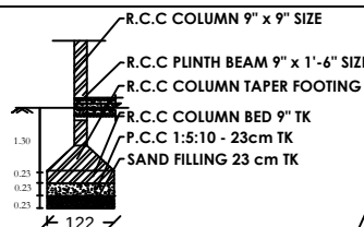
SECTION
