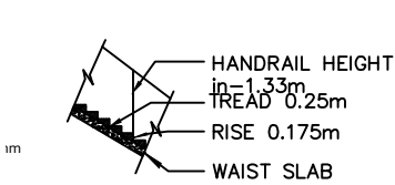
STAIRCASE DETAILS
