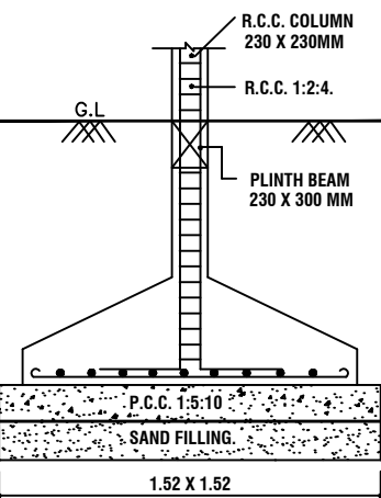
FOUNDATION DETAIL
