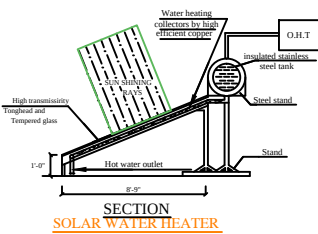
SECTION SOLAR WATER HEATER
