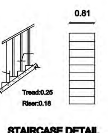
STAIRCASE DETAIL
