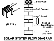
SOLAR SYSTEM FLOW DIAGRAM
