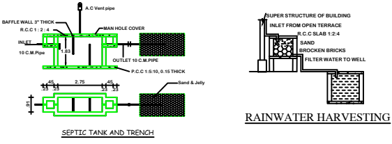
SEPTIC TANK AND TRENCH
