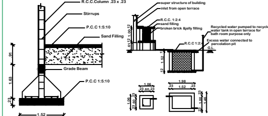
COLUMN DETAIL
