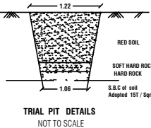
TRIAL PIT DETAILS NOT TO SCALE
