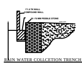
RAIN WATER COLLECTION TRENCH
