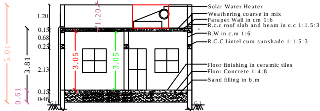
SECTION - "AB "
