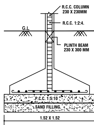
FOUNDATION DETAIL
