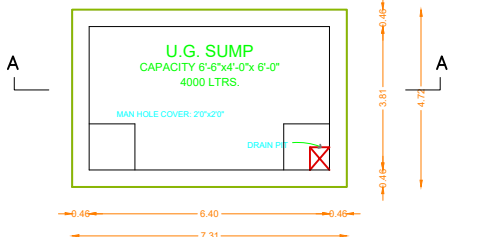
SUMP DETAIL
