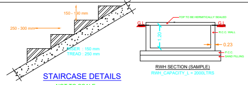
STAIRCASE DETAILS
