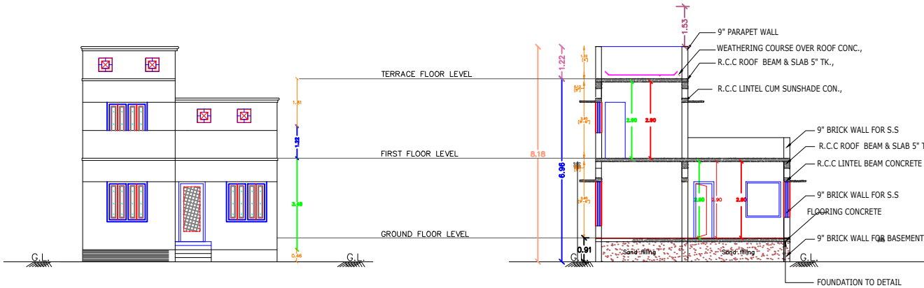
FRONT ELEVATION
