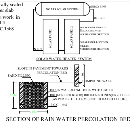
SECTION OF RAIN WATER PERCOLATION BED
