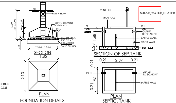
FOUNDATION DETAILS
