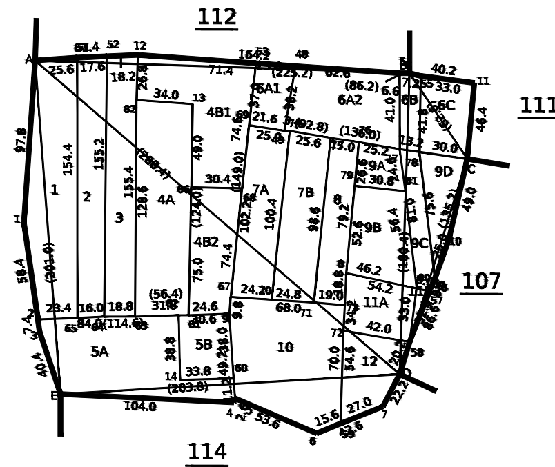
TOPO PLAN
