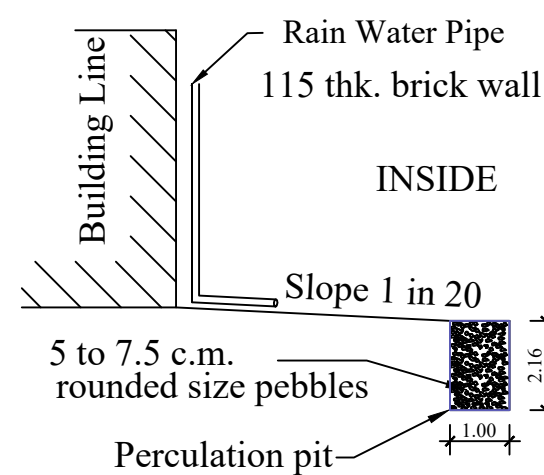
RAIN WATER HARVESTING PERCULATION PIT RWHP CAPACITY L=2000LTRS
