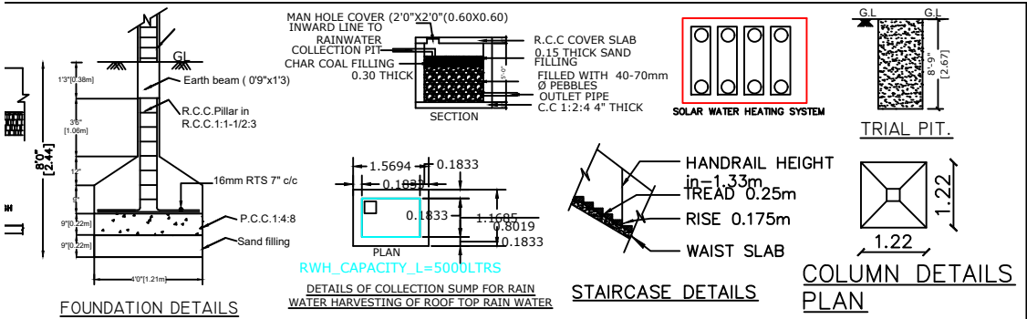
FOUNDATION DETAILS
