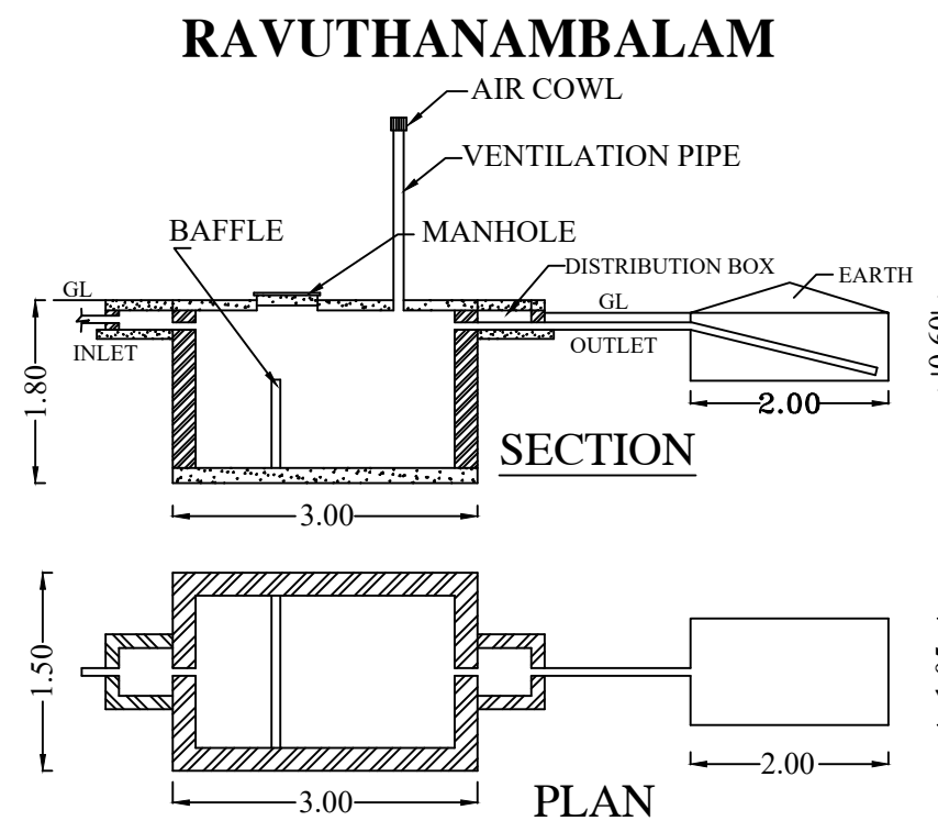
SEPTIC TANK DISPERSION TRENCH
