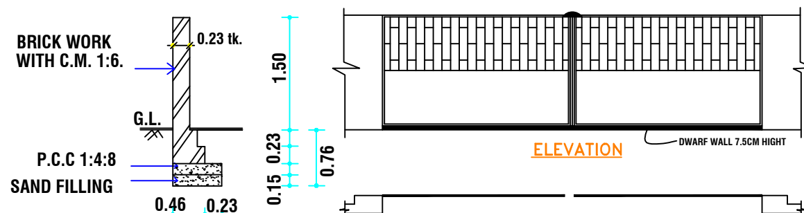
SECTION OF COMPOUND WALL
