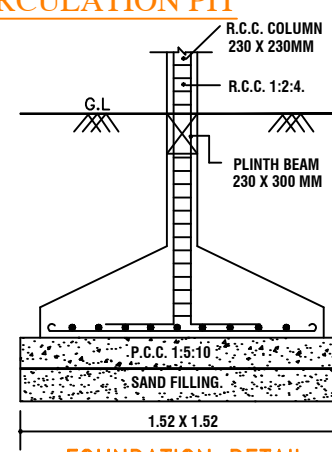
FOUNDATION DETAIL
