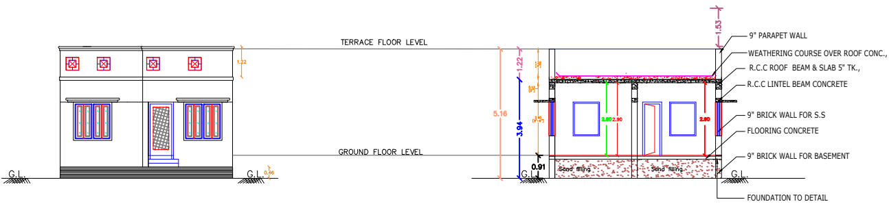
FRONT ELEVATION
