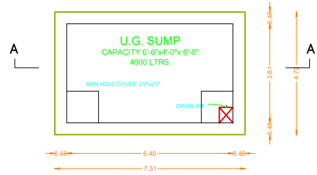
SUMP DETAIL SCALE 1"=4'-0"
