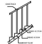
STAIR CASE DETAILS
