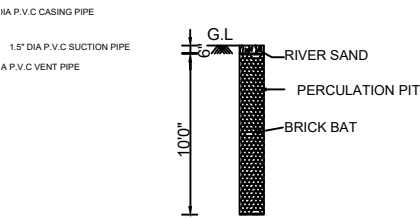
PERCOLATION PIT
