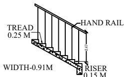
STAIRCASE DETAILS
