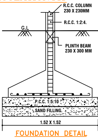
FOUNDATION DETAIL
