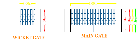
WICKET GATE MAIN GATE
