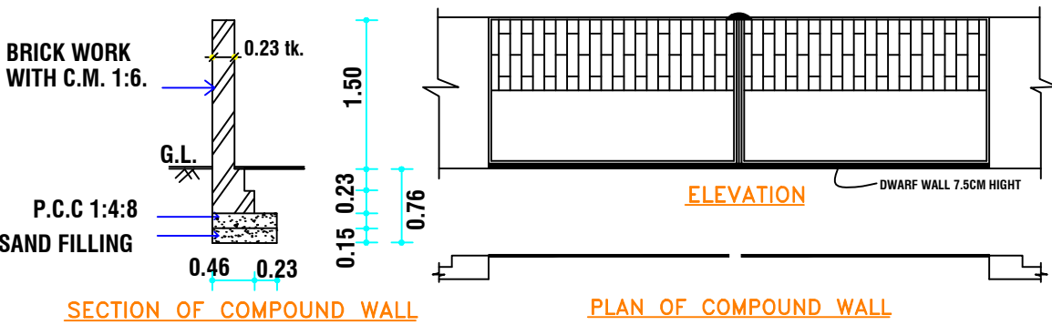
SECTION OF COMPOUND WALL
