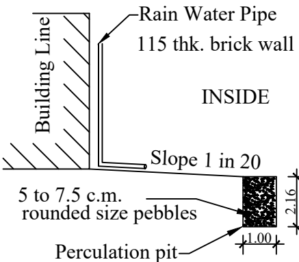
RAIN WATER HARVESTING PERCOLATION PIT
