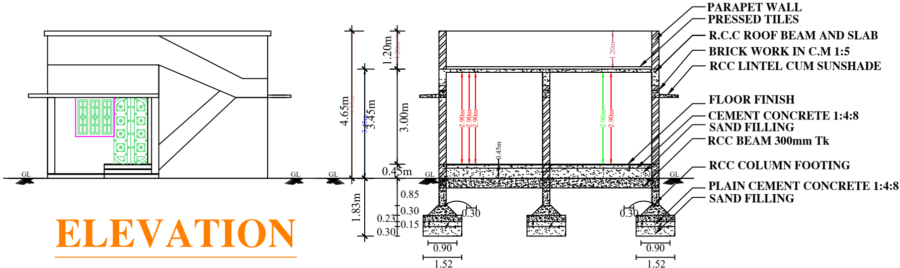
SECTION [A-A]
