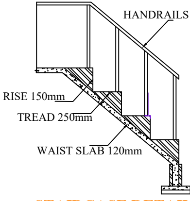
STAIRCASE DETAILS
