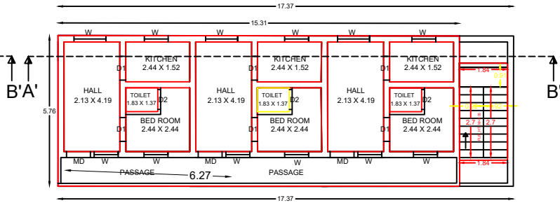
BLOCK-1 FIRST FLOOR
