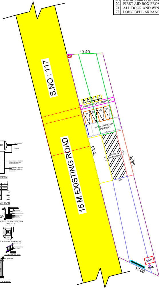
SITE PLAN
