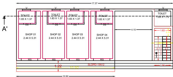
BLOCK-1 GROUND FLOOR
