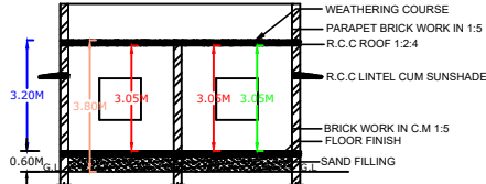
SECTION ON XX
