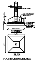
FOUNDATION DETAILS
