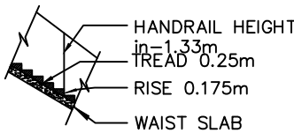
STAIRCASE DETAILS
