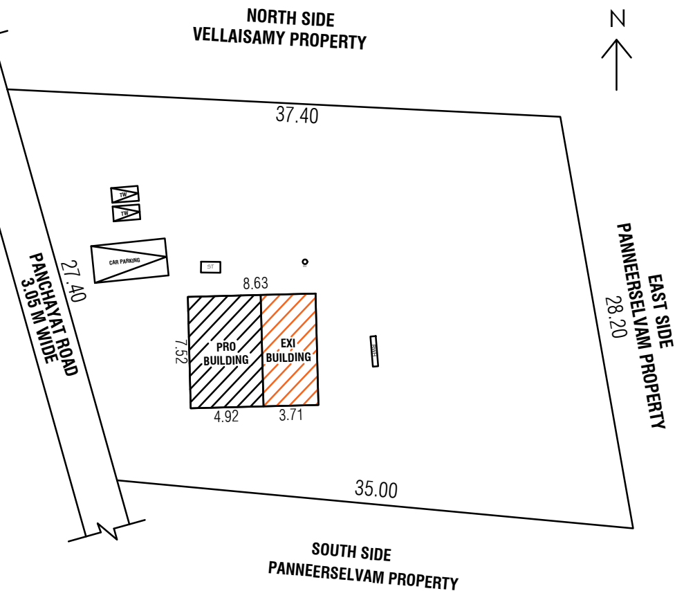
SITE PLAN SCALE - 1:300
